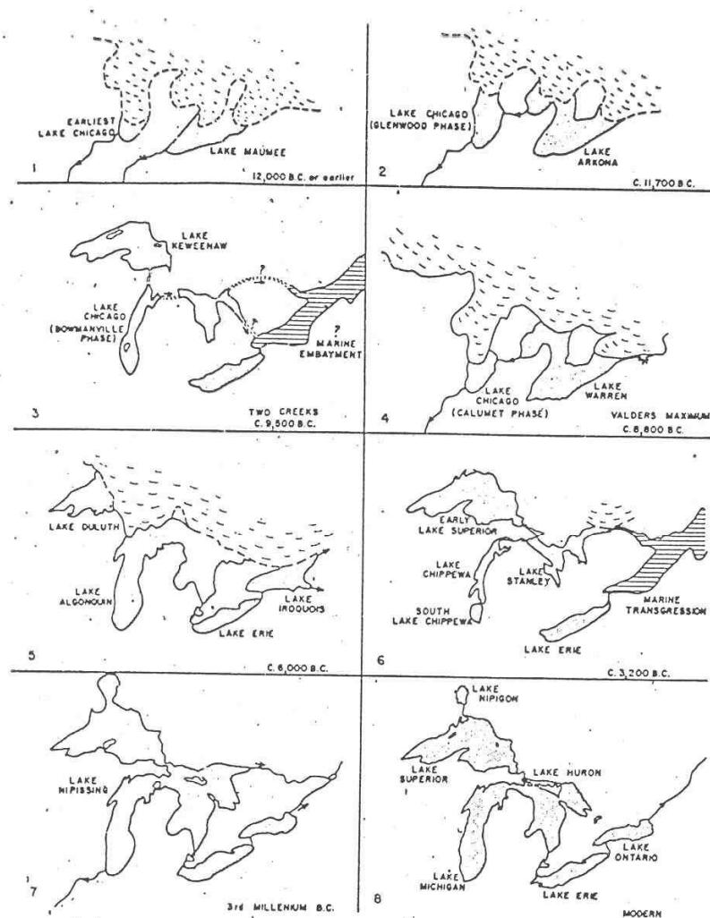
Figure 3-6. The history of the Laurentian Great Lakes. 1, Cary substage; 2, Late Cary; 3, Cary-Valders interstadial, low water in eastern basins, marine transgression in Ontario Basin; 4, Valders maximum; 5, Post-Mankato retreat; 6, Postglacial thermal maximum; 7, Lake Nipissing with triple drainage; 8, Modern lakes. (From Hutchinson, G. E.: A Treatise on Limnology. Vol. 1, New York, John Wiley & Sons, Inc., 1957, after various sources; see Hough, 1958, for details.)
