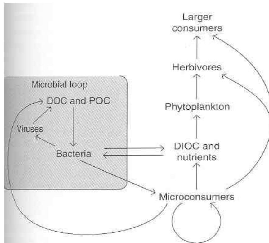
Fig. 9.11 Diagram of the cycling of organic material and nutrients through the phytoplankton and through the microbial loop (shaded box): DOC, dissolved organic carbon; POC, particulate organic carbon; DIOC, dissolved inorganic carbon.
