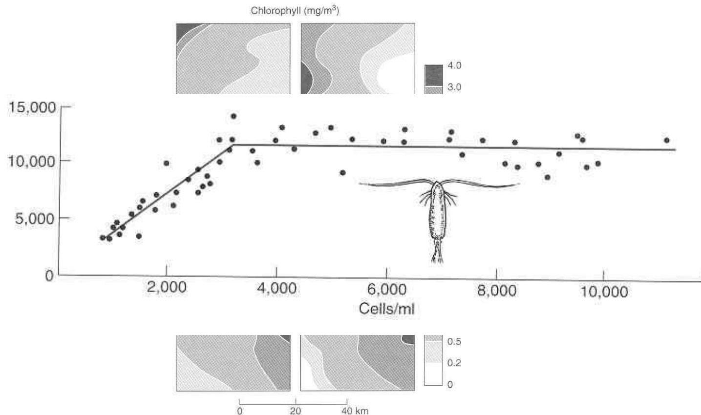
Fig. 9.15 Distribution of chlorophyll a and copepod carbon on a survey in the North Sea, showing an inverse relationship between phytoplankton and zooplankton standing stock. Phytoplankton are most abundant toward the left, whereas zooplankton are most abundant toward the right. (Modified from Steele, 1974.)
