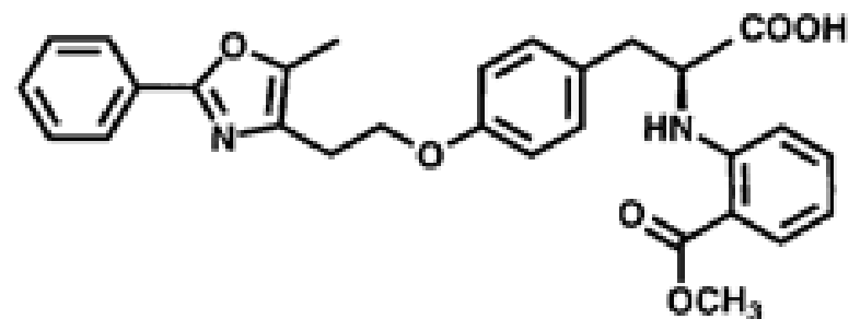
GW 7845
