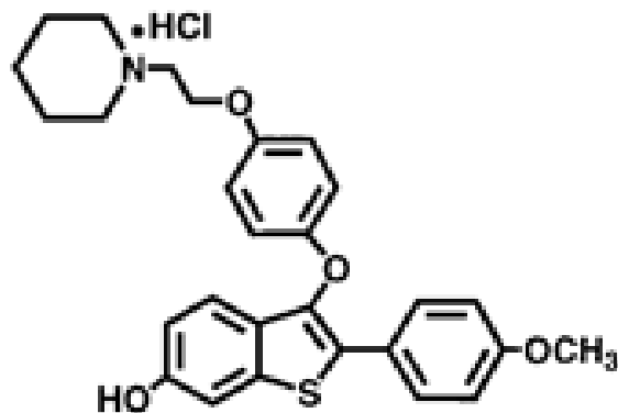
LY353381·HCl
