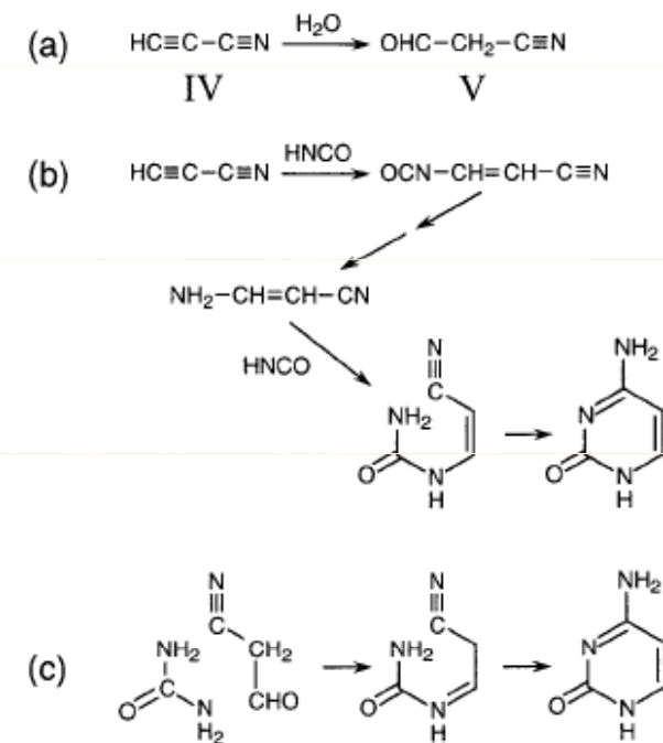
FIG. 3. Steps in proposed prebiotic syntheses of cytosine. (a) The hydrolysis of cyanoacetylene to cyanoacetaldehyde. (b) The reaction between cyanoacetylene and two molecules of cyanic acid. (c) The condensation of cyanoacetaldehyde with urea.
