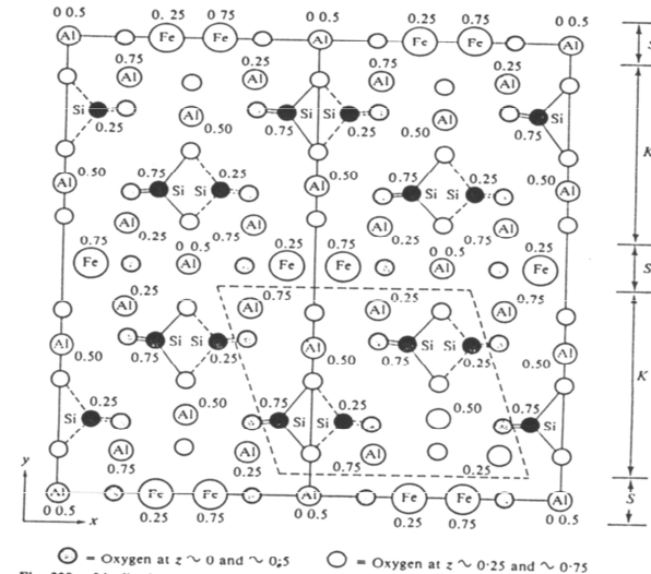
Fig. 329. Idealized structure of staurolite. Two cells are shown projected down z and the kyanite unit cell is also outlined. Alternate blocks of the structure are denoted K (for kyanite) and S respectively (after Náray Szabó and Sasvári, 1958).
