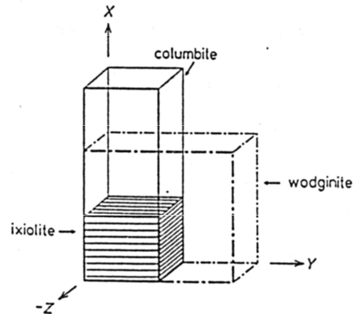
Fig. 11. Orientation and volume relationships among the unit cells of the ixiolite (shaded), columbite (solid rule) and wodginit (broken rule) structures (after Grice et al. 1976).
