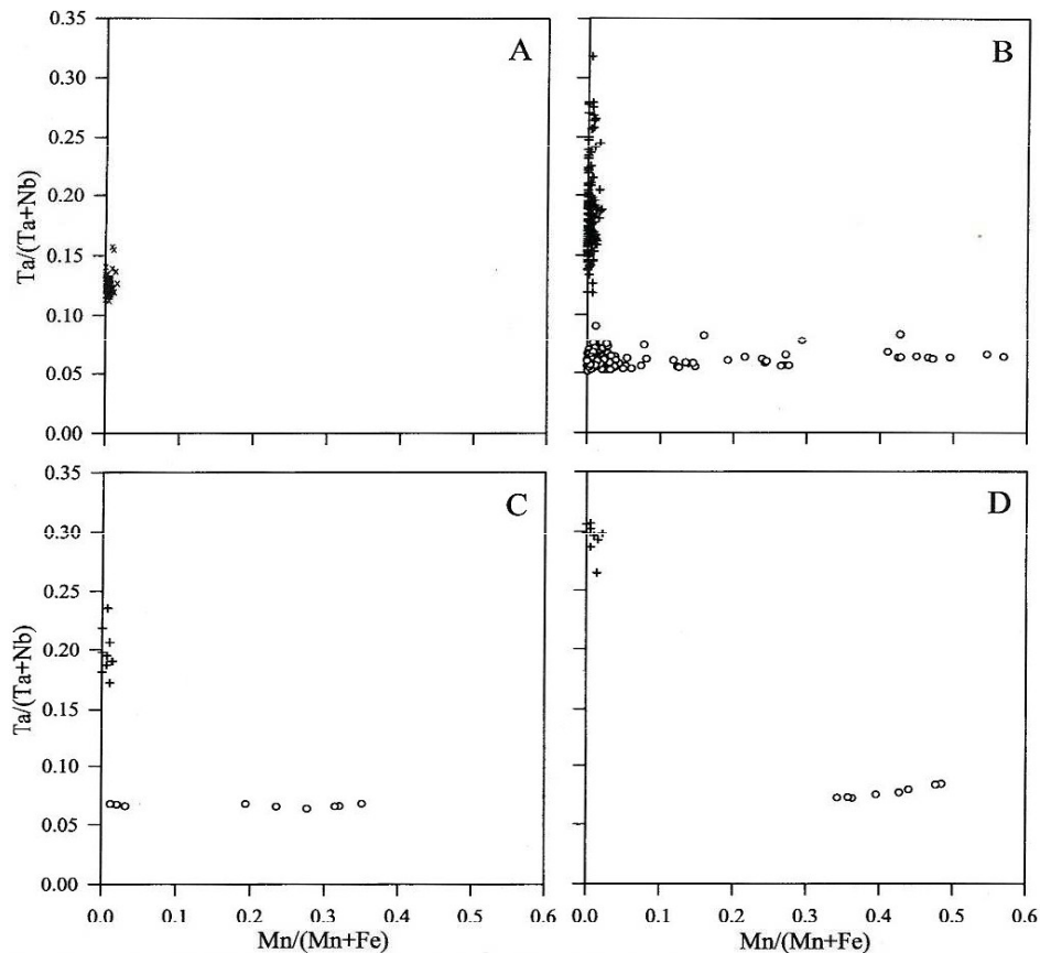
Fig. 2. Compositions of the Věžná I niobian rutile in the columbite quadrilateral (A to D) and in the ternary diagram (Nb+Ta) - (Ti+Sn+Zr+Hf) - (Fe total +Mn+Mg+Sc) (E to H), both in atomic proportions. A and E - primary homogeneous rutile I (cf. Table 1); B and F - depleted rutile I and exsolved titanian columbite (cf. Tables 2 to 4); C and G - niobian rutile II from near Li, Cs-enriched pods (cf. Table 5); D and H - discrete crystals of niobian rutile III and associated titanian columbite from open fissures (cf. Table 6). X - primary niobian rutile, + - depleted niobian rutile, o - exsolved titanian ferrocolumbite.
