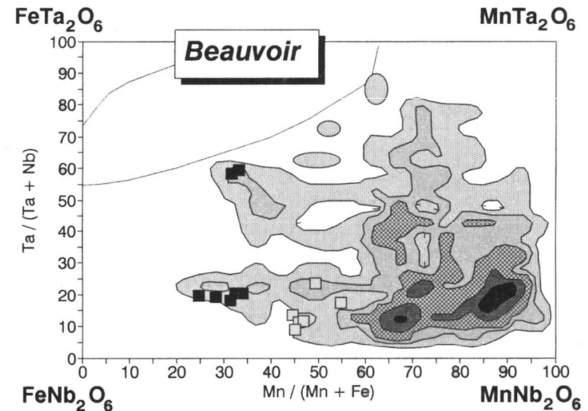
FIG. 2. Quadrilateral diagram of columbotantalite composition from Beauvoir. Filled squares = crystals from B'' veins, open squares = crystals from late quartz veins, fields = distribution of 515 analyses from the Beauvoir granite (Kosakevitch, 1976; Wang et al., 1987; Ohnenstetter and Piantone, 1988). Contour intervals (0.1, 0.5, 1, 2, 3%) are based on a 5 \times 5 grid.
