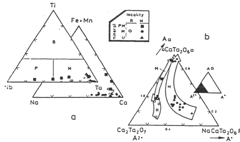
Fig. 3. Triangular plot of divalent A-site cations (mainly Ca), monovalent A-site cations (mainly Na), and A-site vacancies in unaltered and altered microlite samples.
