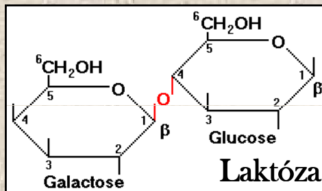
4- O -(beta-D-galactopyranosyl)-beta-D-glukopyranóza
