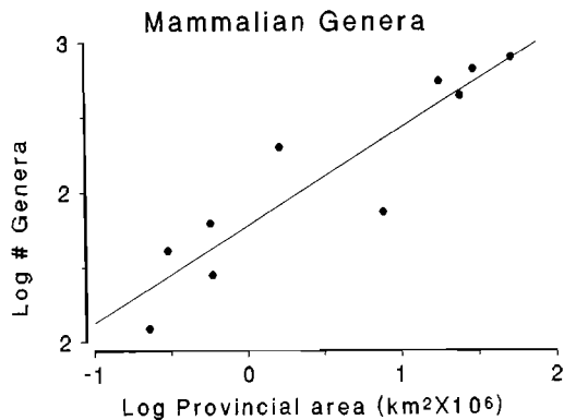
FIG. 8.—Larger biotic provinces have more mammalian genera (modified from Flessa, 1975). Flessa showed that the same relationship holds for families and orders, although their slopes are shallower. The slope for species may even be steeper.
