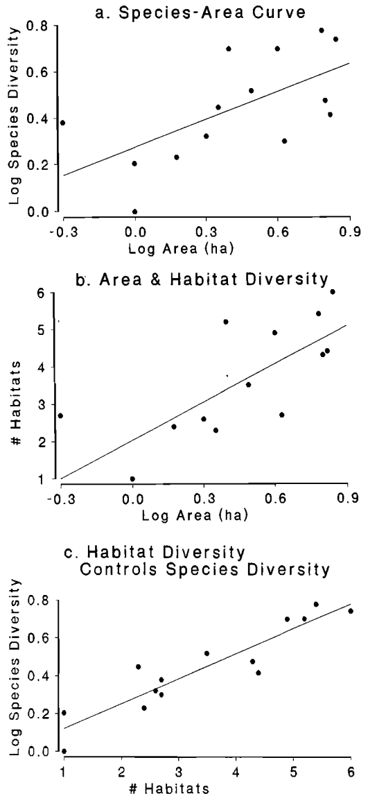
FIG. 10.—Mammal diversity in southeastern Australia fits the number of habitats better than area. (Redrawn from Fox, 1982.)
