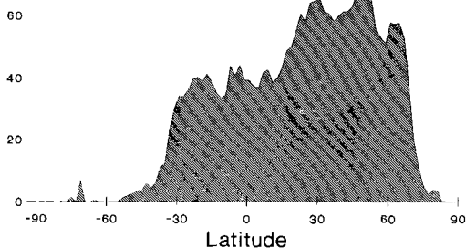
FIG. 4.—An equal area map does not exaggerate the amount of land in the northern hemisphere.
