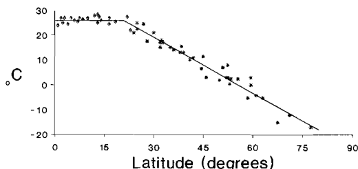
FIG. 5.—In the tropics, average annual temperature varies little with latitude, but it declines linearly outside the tropics. (Data from Terborgh, 1973.)
