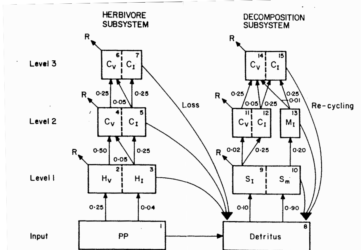
FIG. 1.4. A simple trophic model comparing the organisms of the herbivore and decomposition subsystems (after Heal & MacLean 1975). The symbols are those of the original paper: S = saprovores decomposers; M = microbivore; H = herbivore; C = carnivore; v = vertebrate; i = invertebrate; m = micro-organism; R = loss to respiration; PP = primary production. The transfers linking the compartments are the fractions transferred at any one linear run of the model.
