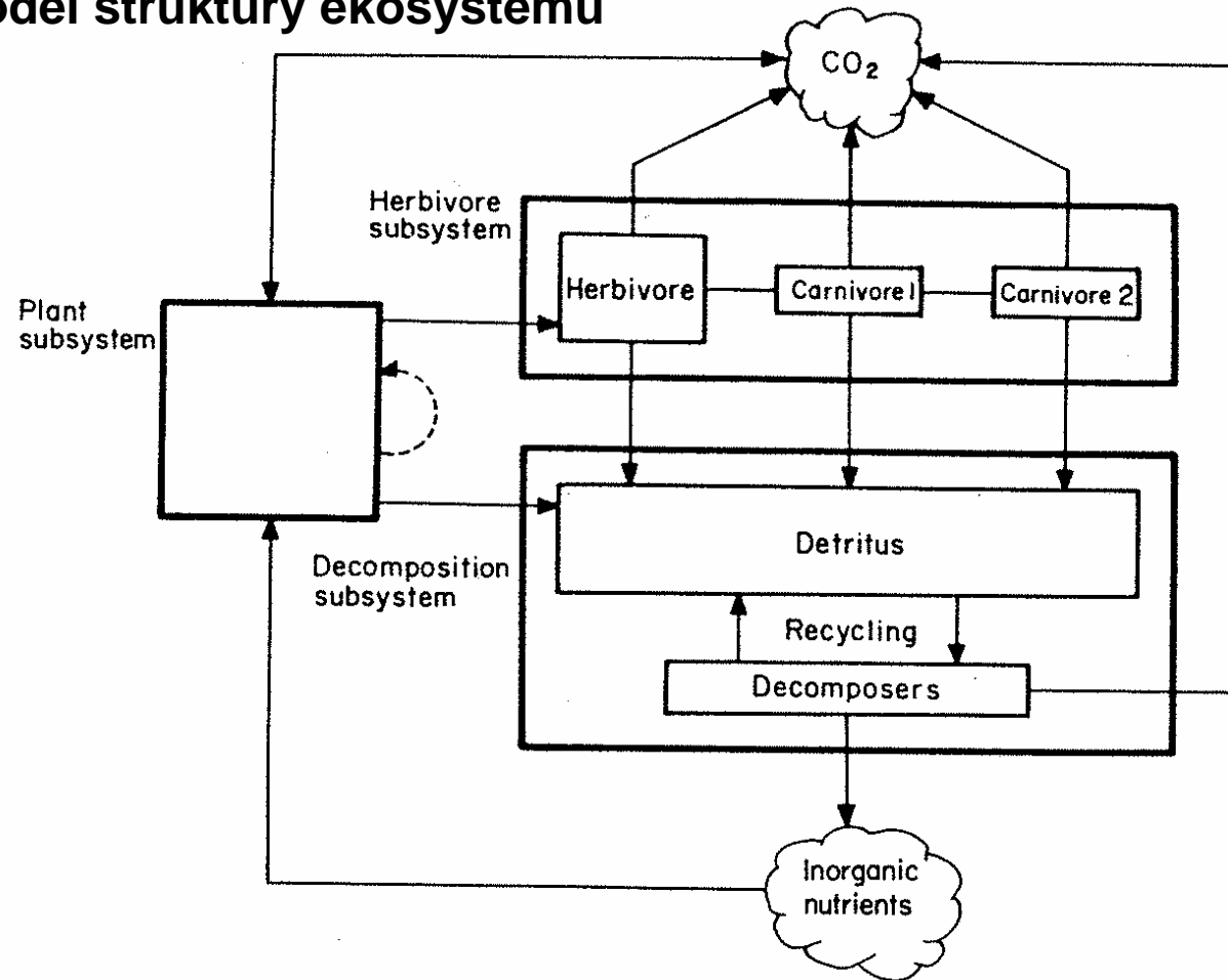
FIG. 1.3. A general model of ecosystem structure. The three subsystems are shown together with their main components. The major pathways of transfer of matter within the ecosystem are shown by the arrows. Organic matter pools are shown as rectangles, inorganic as 'clouds'. Note in particular the links between the herbivore and decomposition subsystems, the recycling of matter within the decomposition subsystem and the nett storage of matter that may occur within the plant subsystem (broken arrow).
