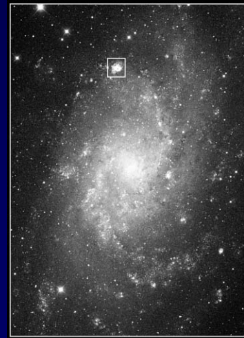
NGC 604 in Galaxy M33
