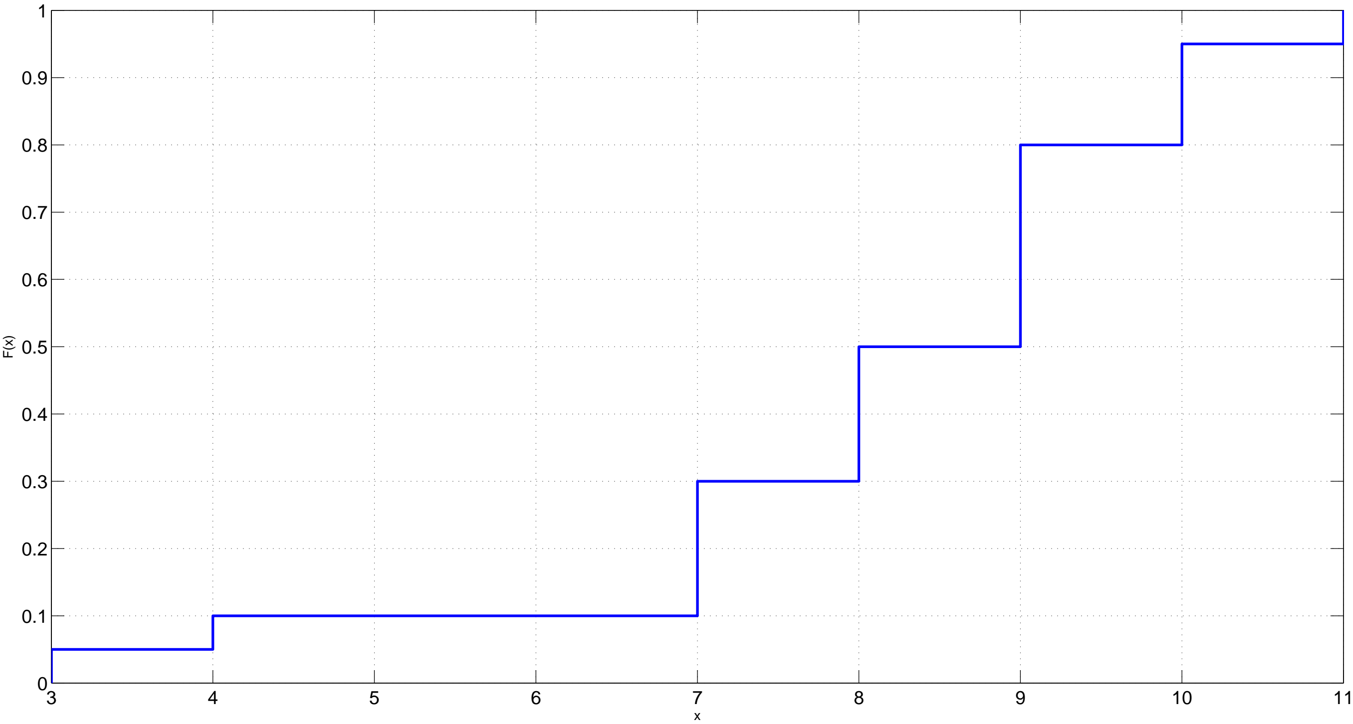
Empirical CDF
