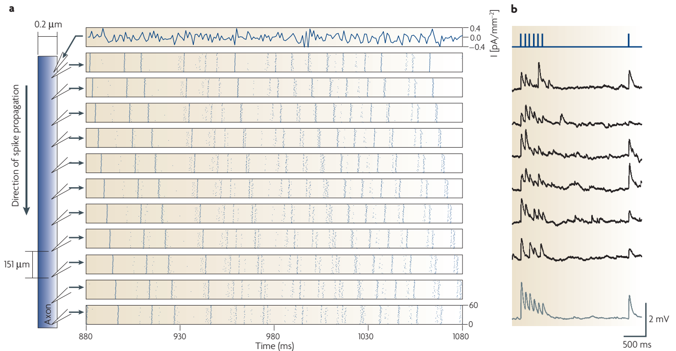
Figure 2 | Examples of cellular noise. a | Channel noise as a source of trial-to-trial variability in action potential (AP) propagation. Stochastic simulations of the response of a 0.2 μm diameter CNS axon (comparable with a cerebellar parallel fibre) in response to repeated identical current stimuli and initial conditions are shown. The only source of variability is the stochastic opening and closing of a million individually simulated ion channels. Spike trains were triggered by a time-varying current stimulus (top plot). Spike raster plots for each measurement site are shown, from the soma (second-from-top plot) down to the most distal part (the axon; bottom plot). In each raster plot, the precise timing of spikes is marked by dots, which are stacked over each other for each repeated trial (there were 60 trials). The shift of the overall spike pattern across rows reflects the average propagation speed of the APs. The raster plot of the somatic measurement reflects spike-time variability from AP initiation. Owing to channel noise, the spike-time variability rapidly increases the further the AP propagates, and it eventually reaches millisecond orders. b | Trial-to-trial variability of synaptic transmission measured in vitro by paired patch-clamp recordings in rat somatosensory cortex slices. Six consecutive postsynaptic responses (black traces) to an identical presynaptic-stimulation pattern (top trace) are shown, along with the ensemble mean response (grey trace) from over 50 trials. Part a modified from REF. 65. Part b modified, with permission, from REF. 77 © (2006) American Physical Society.
