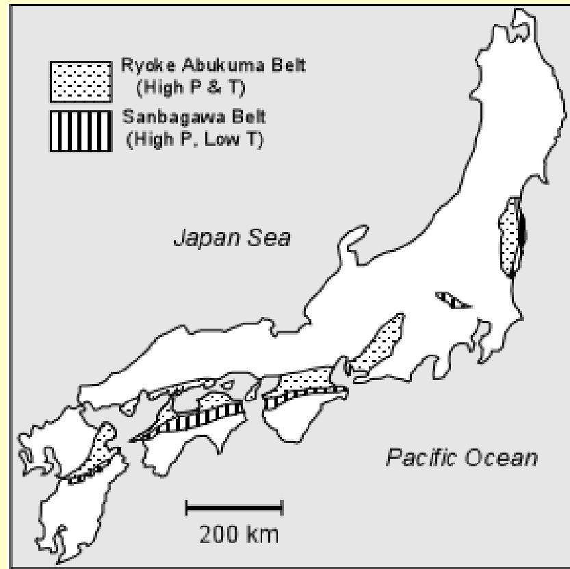
After Miyashiro (1961)
