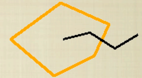
Linestring/Polygon
