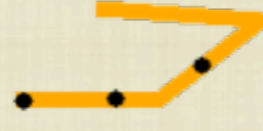
Multipoint/Linestring
