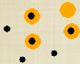
Multipoint/Multipoint
