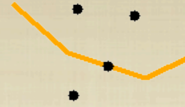
Multipoint/Linestring
