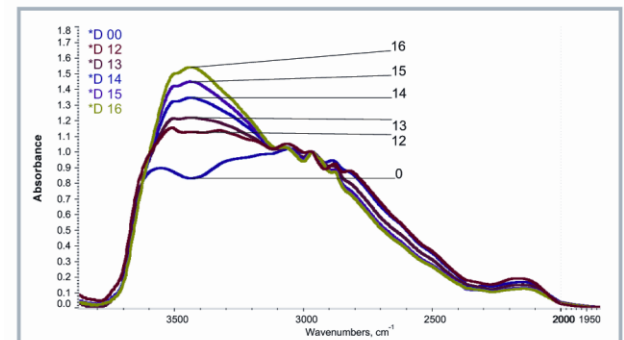
Figure 3. Fragments of transmission spectra of wool fibres in the 3650-3150\text{ cm}^{-1} range of IR absorption by groups with the O-H, N-H oscillator. Spectrum shapes change in relation to the intensity of plasma treatment (samples 0, 12, 13, 14, 15 and 16).
