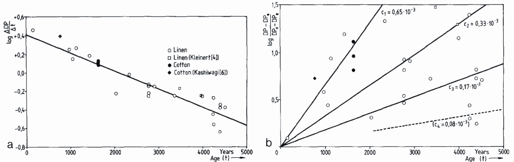
Fig. 2. (a) Relationship between \log \Delta DP / \Delta t and the age t of the linen samples according to the regression equation \log \Delta DP / \Delta t = 0.41 - 1.96 \cdot 10^{-4} \cdot t . (b) Dependence of the DP from the age of the linen samples according to the relationship DP - DP_c = (DP_0 - DP_c) \cdot \exp. (-ct)
