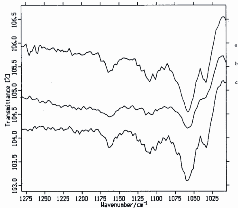
FIG. 6. Stack-plot of the infrared spectra for crystalline material (as KBr disks) from ( a and b ) Egyptian mummy linen samples, and ( c ) Kasr-el-Yahud linen sample; wavenumber region 1000–1280 \text{cm}^{-1} .
