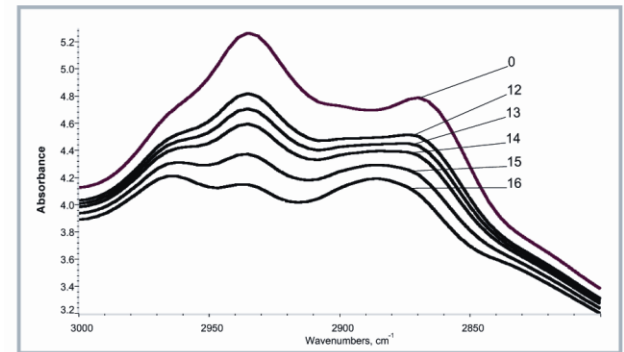
Figure 1. Fragments of transmission spectra of wool fibres in the 3000-2800\text{ cm}^{-1} range of IR absorption by groups with the C-H oscillator; 0 - spectrum for wool not modified with plasma, 12, 13, 14, 15, 16 - IR spectra for wool samples treated with LTP, with an increasing value of the electric power of the plasma and constant time (Table 2).
