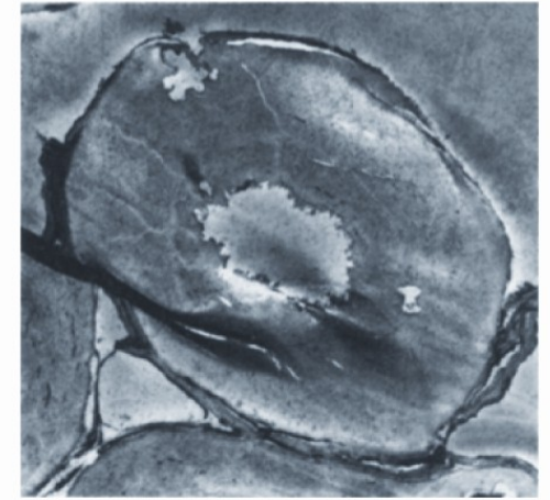
Fig. 1. Cross section of a linen fiber from a mummy wrapping being about 4 250 years old (6th dynasty, Giza, tomb of Idu). At the lumen side and also within the cell wall the beginning of a degradation is visible. Transmission electron micrograph, magnification 5400 ×
