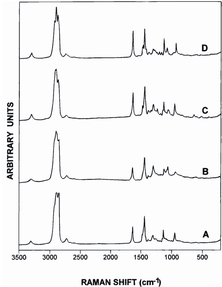
FIG. 5—Raman microprobe spectra (632.8 nm excitation) of a set of nylon fibers of different molecular structure. (A) nylon-6,12 (AO464); (B) nylon-6,11 (AO302); (C) nylon-6,6 (AO330); (D) nylon-6 (AO208).
