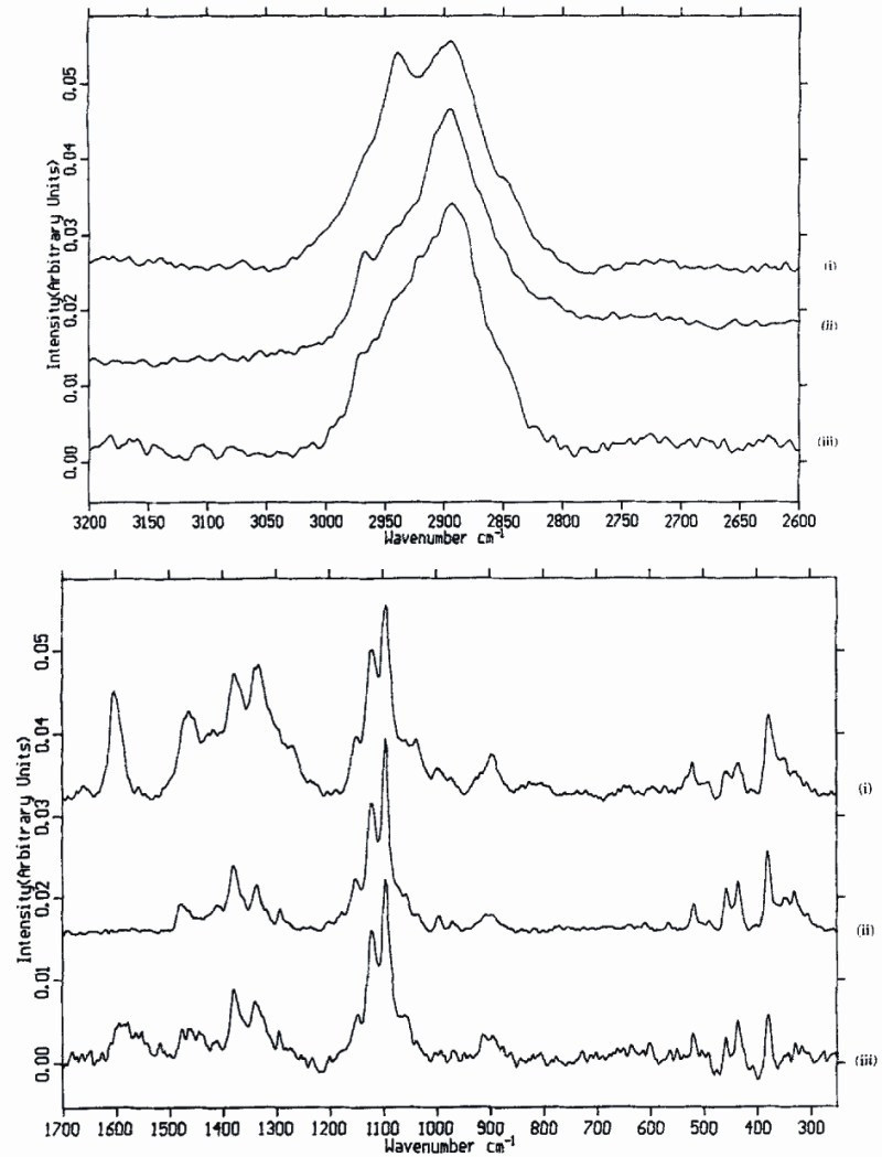
Fig. 2. FT-Raman spectra of soft bast fibres, (i) jute; (ii) ramie; and (iii) flax: (a) 2600–3200 cm -1 region; (b) 200–1700 cm -1 region: 1064 nm excitation, spectral resolution 4 cm -1 , 2000 scans accumulated, laser power 40 mW.
