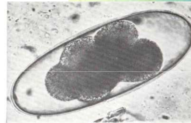
FIG. 57—Ovum of Marshallagia marshalli . x 410. x 410
