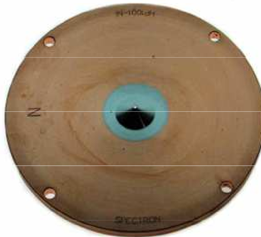
Sampling cone
