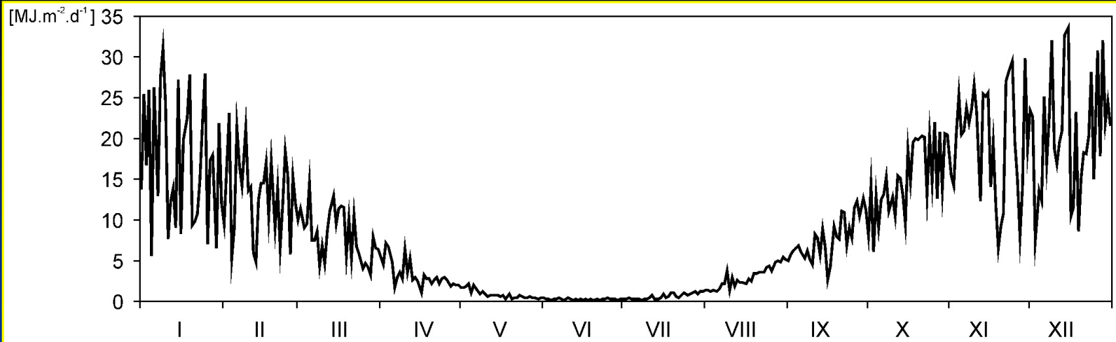
Daily sums of global Sun radiation - annual regime of 2005; J. G. Mendel Station
