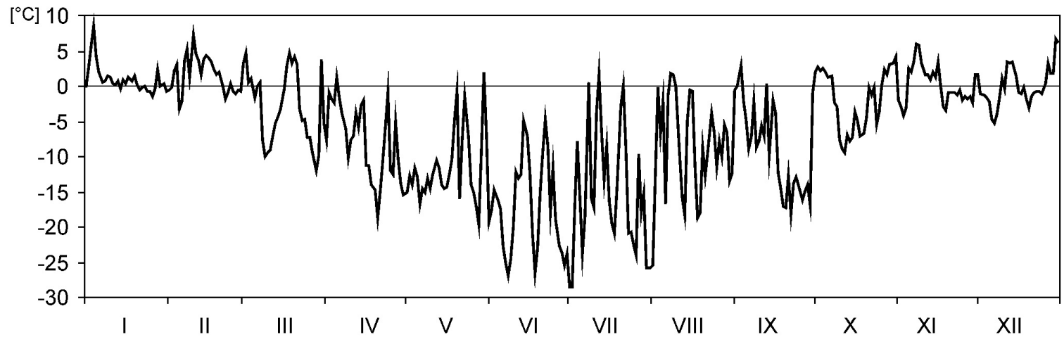
Mean daily temperatures - annual regime of 2005; J. G. Mendel Station
