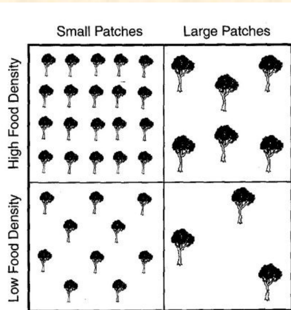
FIGURE 3.7 Different patterns of spatial distribution of potential food resources.
