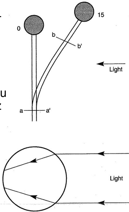
Figure 4.5 Phototropism of the sporangiofore of Phycomyces . A, Growth and curvature of a sporangiofore during its final phase of elongation, after sporangium formation. The position of the sporangiofore at the onset of unilateral illumination (0) and 15 minutes later (15) is shown. It can be seen that for curvature to occur wall growth has to be greater on the far side (a–b) of the sporangiofore than on the side near the light source (a'–b'). B, A diagrammatic section of the sporangiofore (as for example at a–a') showing how light is focused on the far side of the sporangiofore.
