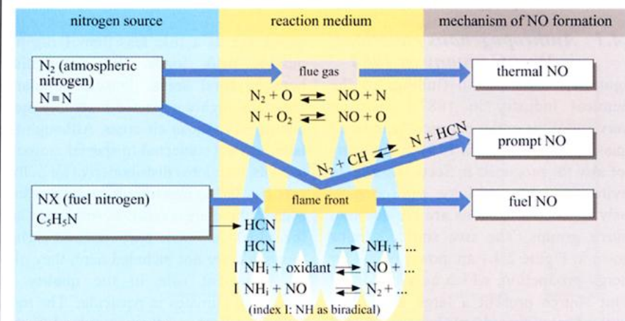
1. Mechanisms of NO formation
