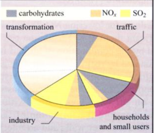
1. Fractions of individual air pollutants by emitter
