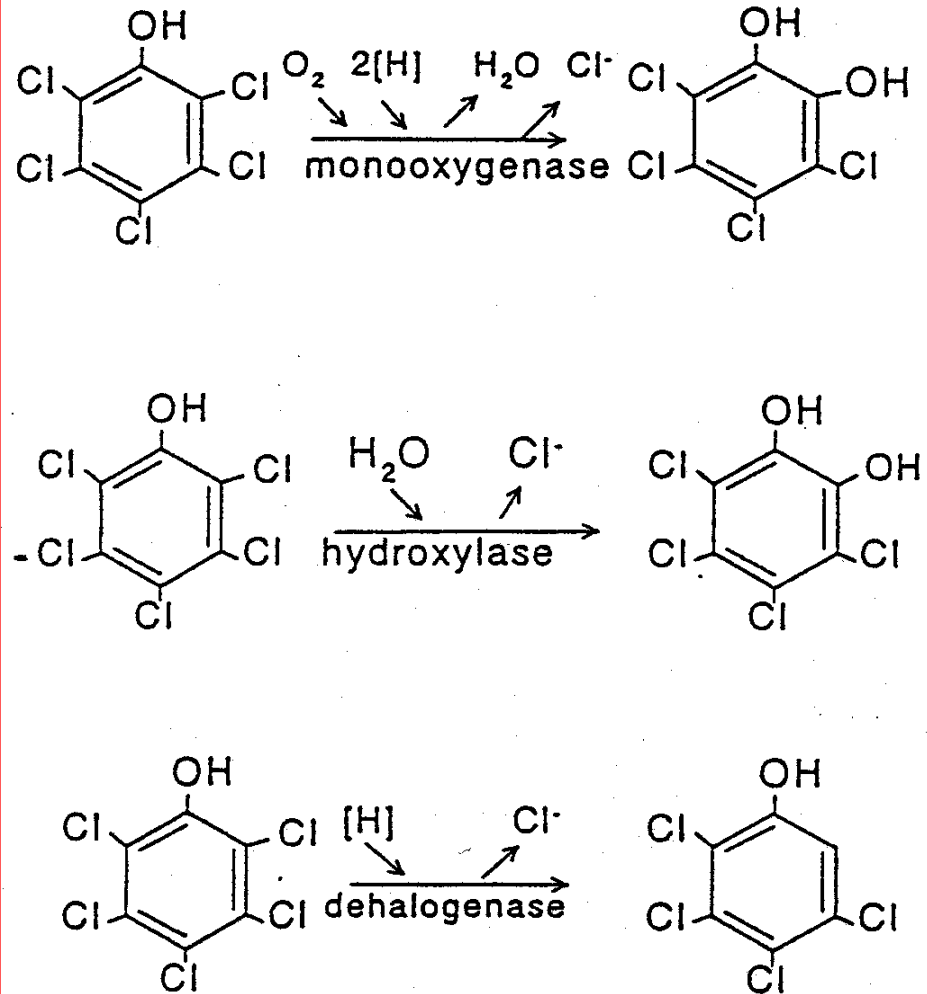
Fig. 1. Pathways of PCP degradation.
