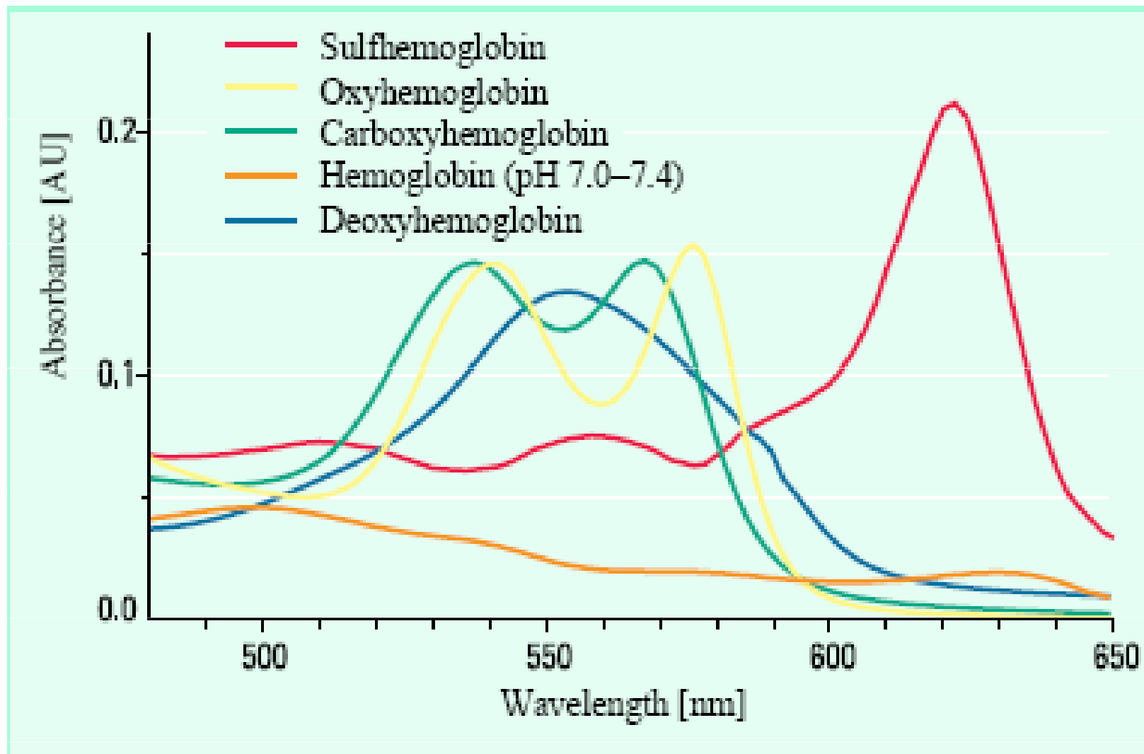
Figure 15 Absorption spectra of hemoglobin derivatives
