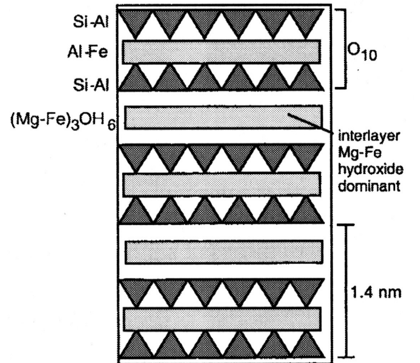
chlorite
