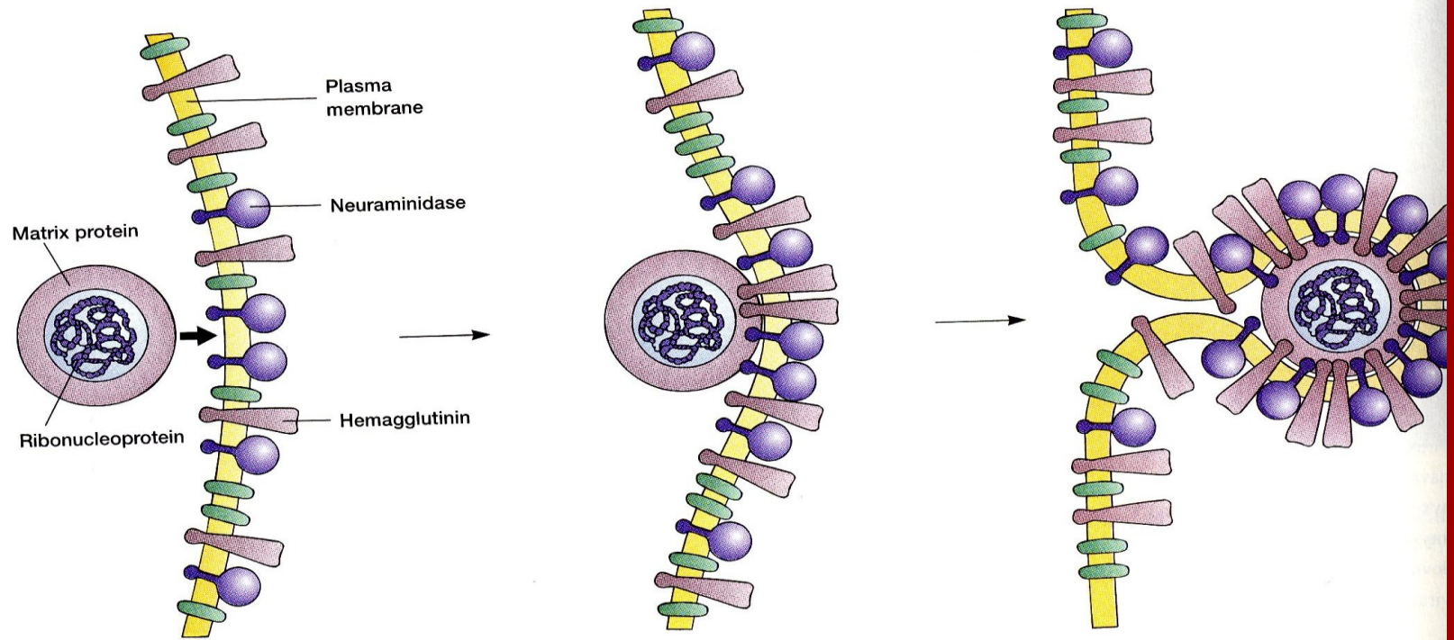
Figure 18.8 Release of Influenza Virus by Plasma Membrane Budding. First, viral envelope proteins (hemagglutinin and neuraminidase) are inserted into the host plasma membrane and binds to it. At the same time, the nucleocapsid approaches the inner surface of the membrane. Finally, the plasma membrane buds to simultaneously form the virion envelope and release the mature virion.
