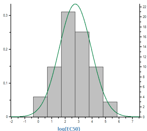
Parameters of the normal distribution
