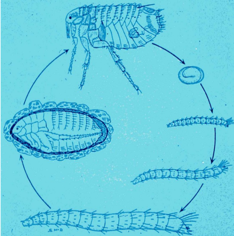
Life-cycle of a flea
