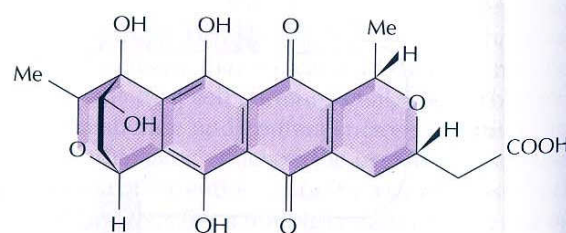
Dihydrogranatirhodine
