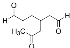
3-(2-oxopropyl)hexan-1,6-dial
