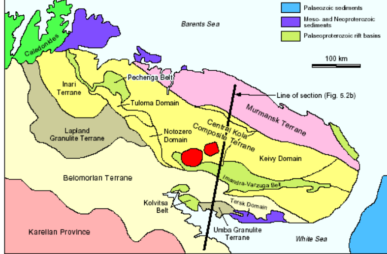
Figure 5.2a: Tectonostratigraphic terranes in the Lapland-Kola Orogen from Balagansky and Glaznev (pers. comm. 1994) and incorporating data from Marker (in Blundell et al., 1992).
