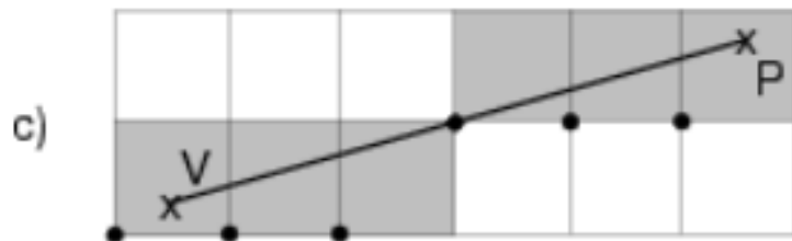
vector-to-raster-conversion
