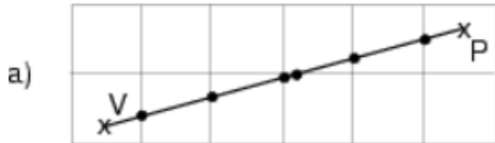
line intersection
