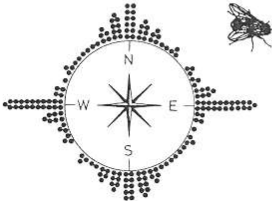
geomagnetic field
