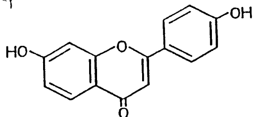
dihydroxyflavon
