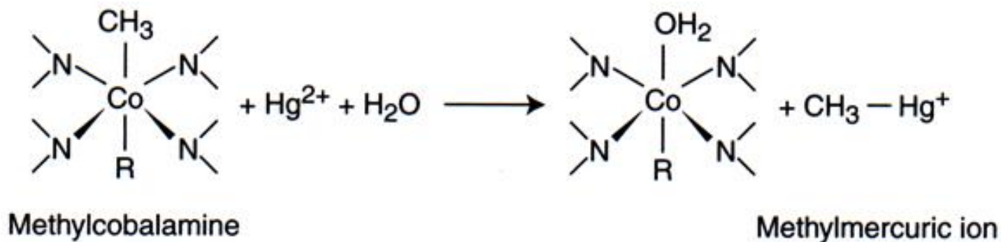
FIGURE 8.2 Methylation of inorganic mercury by methylcobalamin. From Crosby (1998).
