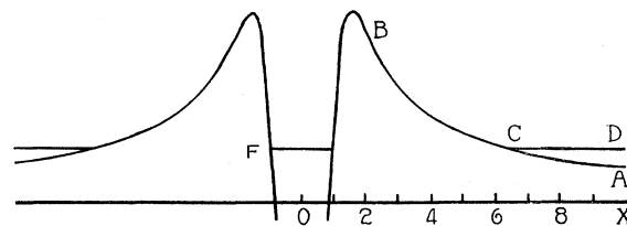
Fig. 5. The unit of abscissas is 10^{-12} cm. The horizontal line gives the energy of the \alpha -particle emitted by uranium, 6.5 \times 10^{-6} ergs.
