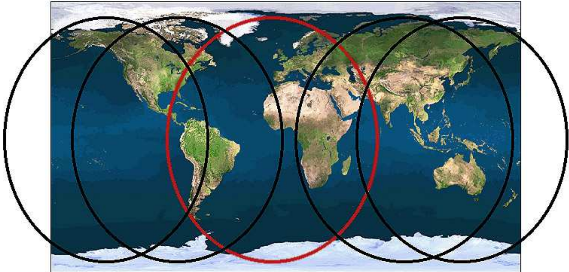
GOES-9
