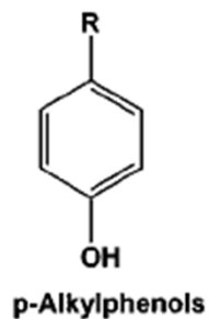
Figure 2 Structures of some xenoestrogens.
