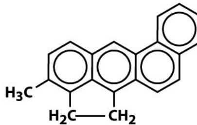
3-methylcholanthrene
