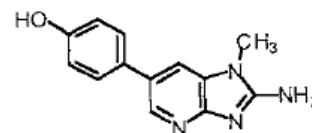
4'-hydroxy-PhIP
