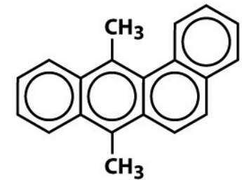
7,12-dimethylbenz[ a ]-anthracene
