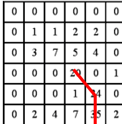
Flow accumulation
