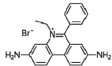
etidium bromid
