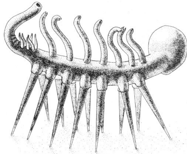
Hallucigenia
