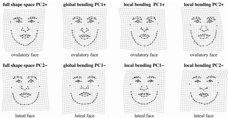
Fig. 2. TPS deformation grids; PCA in full shape space (first column; PC2, explained variance 12.17%); PCA for global bending patterns (second column; PC1, 47.16%), and PCA for local bending patterns (last two columns; PC1 and PC2, 14.46% and 12.24%, resp.)
