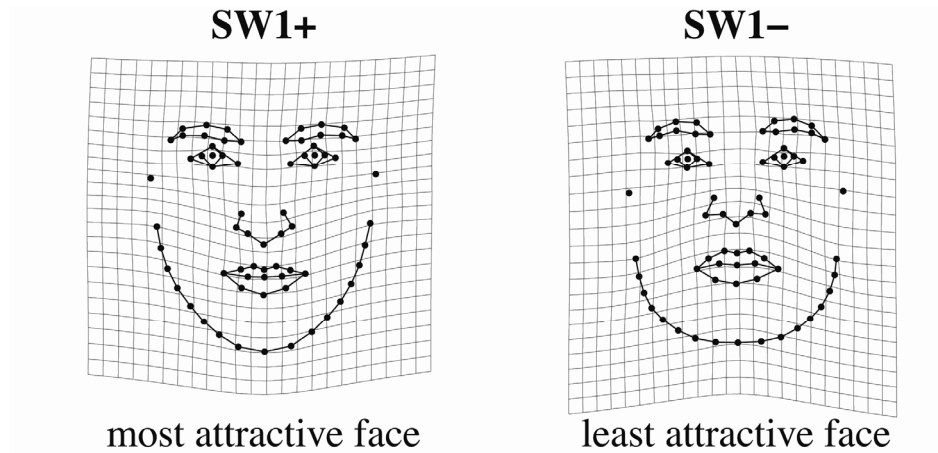
Fig. 3. TPS deformation grids of PLS in SW1 (ovulatory faces only, explained variance 54.84%, Pearson product-moment correlation coefficient of attractiveness ratings and shape coordinates = 0.622, calculated based on SW1 scores)
