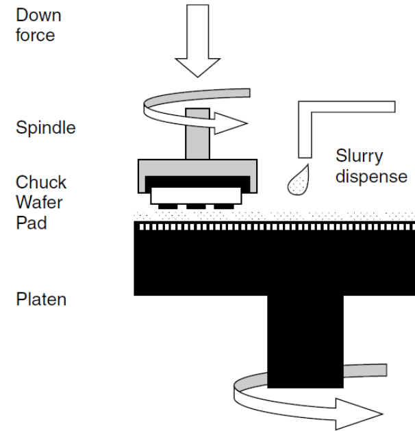
Figure 16.2 Schematic structure of a rotary CMP equipment
