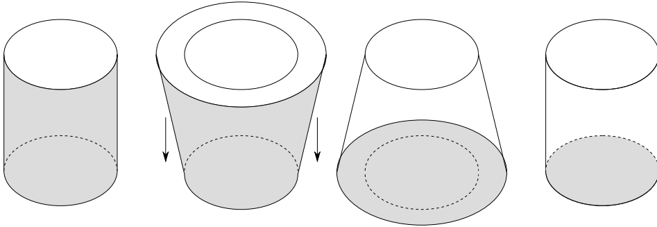
FIGURE 10.4. Homeomorphism (D^n \times I, D^n \times \{0\} \cup S^{n-1} \times I) \rightarrow (D^n \times I, D^n \times \{0\})
