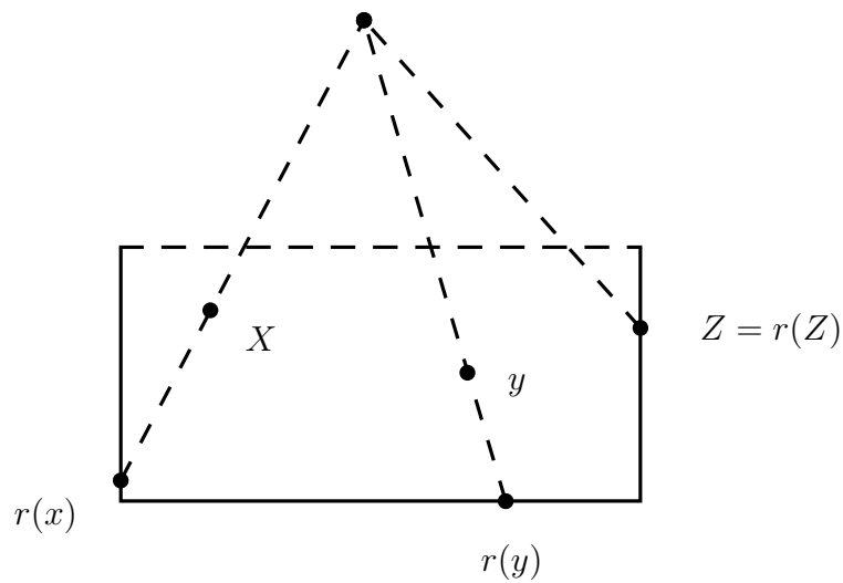
FIGURE 1.4. Retraction D^1 \times I \rightarrow D^1 \times \{0\} \cup S^0 \times I
