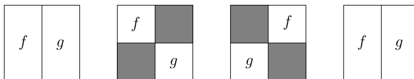
FIGURE 10.1. f + g \sim g + f
