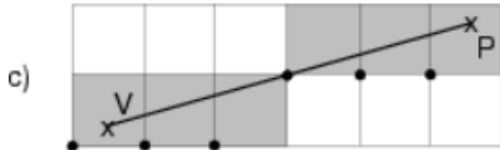
vector-to-raster-conversion
