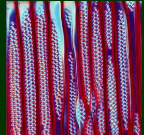
Araucaria – tracheidy
