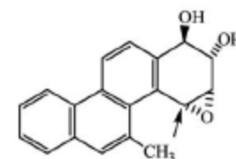
1R,2S,3S,4R-5MC-diol epoxide
