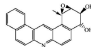
3S,4R,1R,2S-DB[a,j]A-diol epoxide
