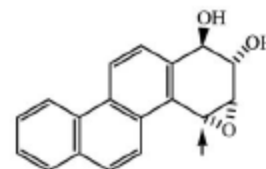
1R,2S,3S,4R-CHR-diol epoxide
