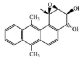
3S,4R,1R,2S-DMBA-diol epoxide
