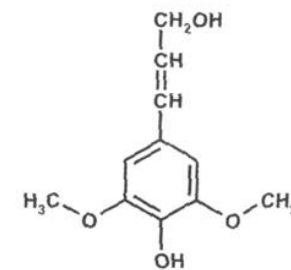
Sinapyl alcohol
