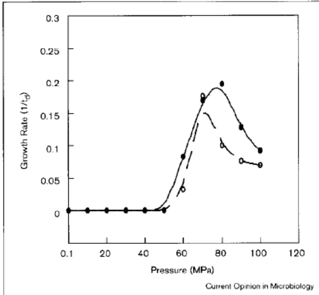
Growth profiles of barophilic bacteria strains DB21MT-2 (-●-) and DB21MT-5 (-○-) at 10°C.
