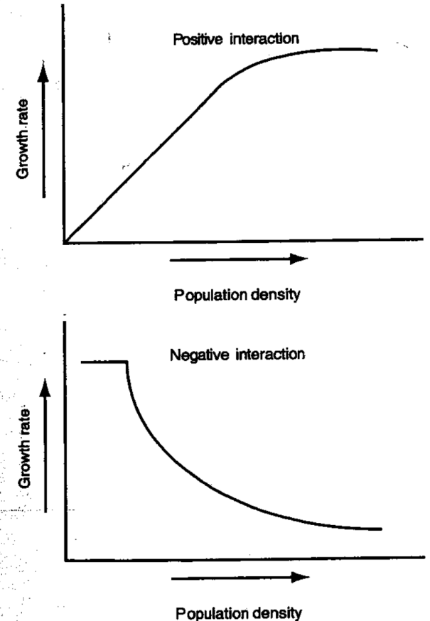
Figure 3.1 Effects of independent positive and negative interactions on growth rate within a single population with increasing population density.
